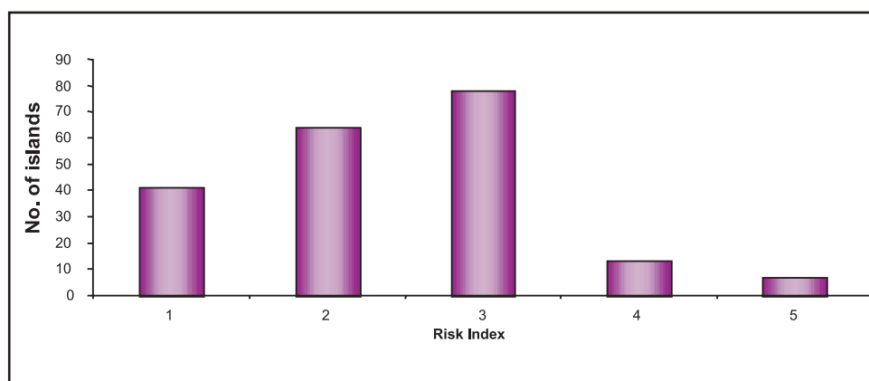
Figure 39: Distribution of Tsunami Risk to Physical Assets across Islands
