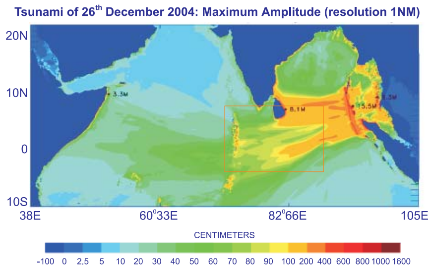
Figure 11: Maximum Computed Amplitude through Numerical Modeling at Alaska Tsunami Warning Center
