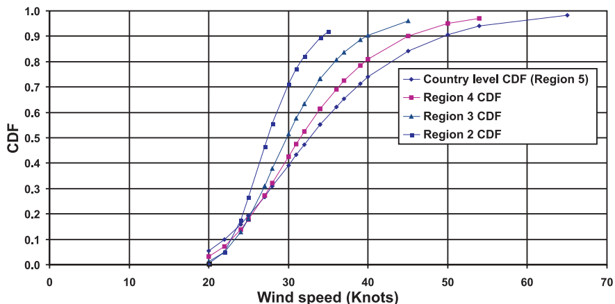
Figure 18: Wind speed Cumulative Distribution Functions by Region
