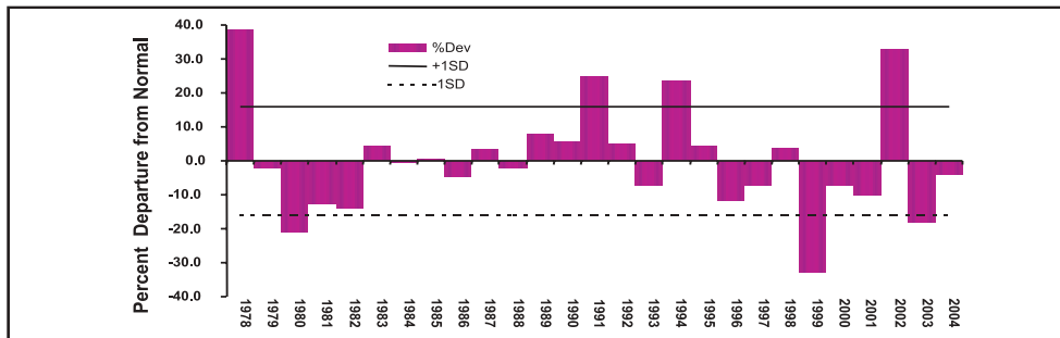
Figure 26: Excess, Normal and Deficient Rainfall Years of Gan
