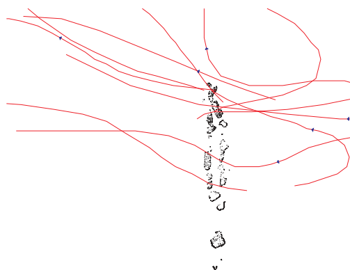
Figure 14: Tracks of Cyclones affecting Maldives, 1877-2004
