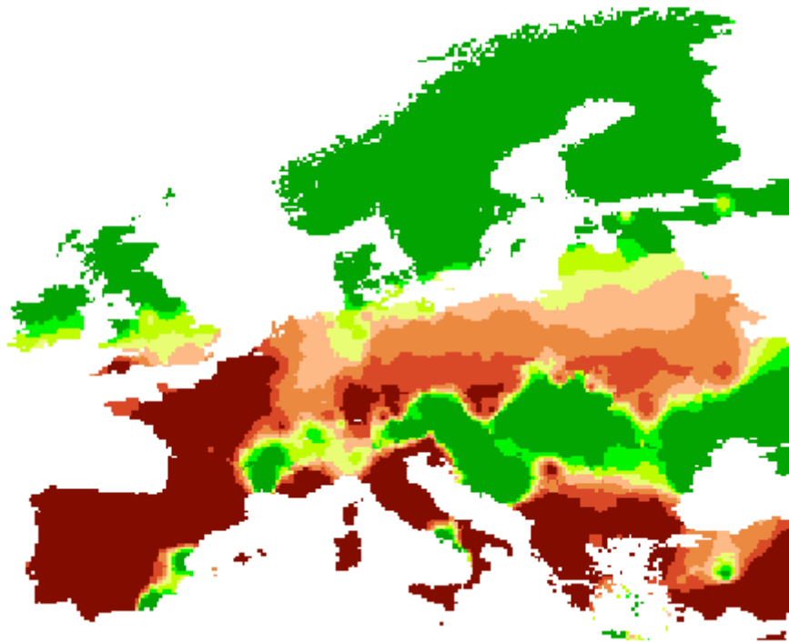
Figure 8. Agriculture: crop yield changes of the 5.4°C scenario (2080s)
