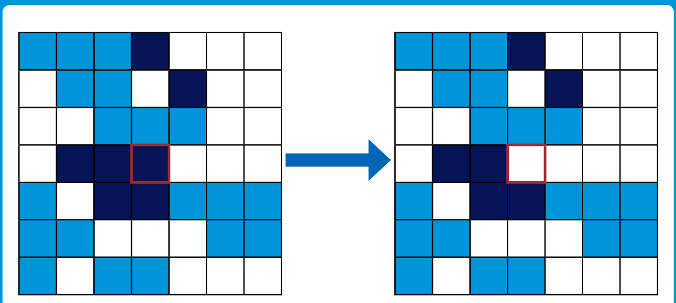
Figure 8: Spatial filtering ( 7 \times 7 filter window) uses a major class algorithm to eliminate cloud pixels at the centre of the matrix
