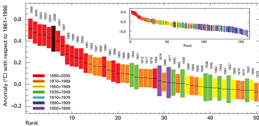
Figure 3 – Global ranked surface temperatures for the warmest 50 years; inset shows global ranked surface temperatures from 1850. The size of the bars indicates the 95-per cent confidence limits associated with each year. The source data are blended land surface air temperature and SST from the HadCRUT3 series (Brohan et al, 2006). Values are simple area-weighted averages for the whole year. [Source: The Met Office Hadley Centre, UK, and Climatic Research Unit, University of East Anglia, UK]
