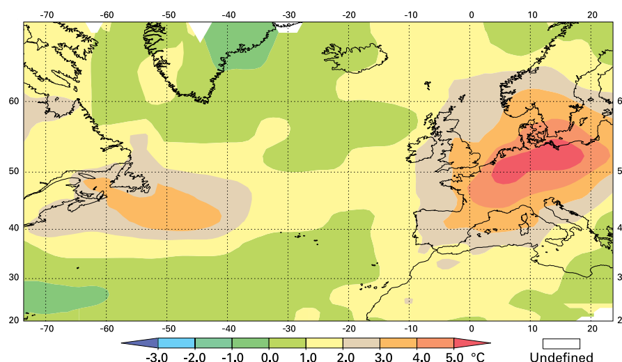
Figure 4 – Monthly air temperature anomalies showing departures in degrees Celsius, 1961–1990 base during the July 2006 summer heat wave over Central Europe [Source: Deutscher Wetterdienst, Germany]
