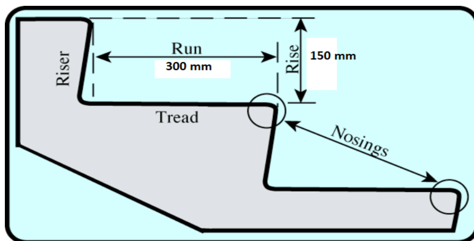
Riser and Tread of Staircase
