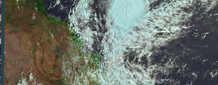
Tropical Cyclone Penny 24 December 2018 – 4 January 2019
