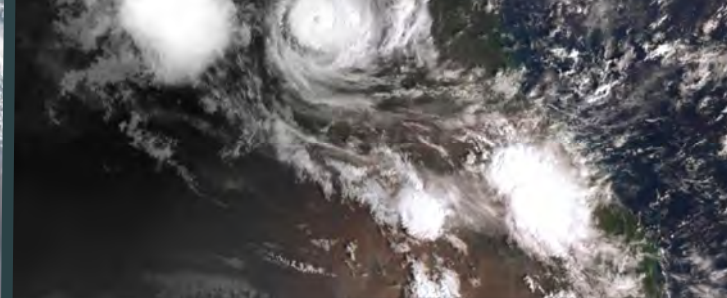
Tropical Cyclone Owen 9-17 December 2018
